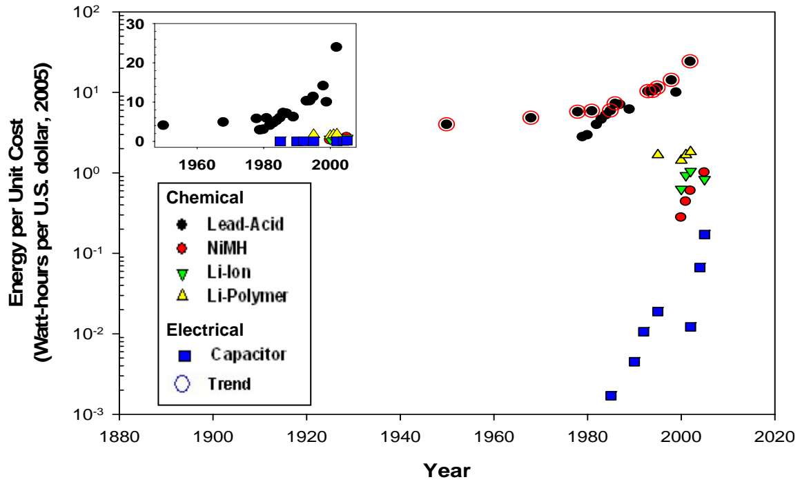
Figure 2 Historical progresses in energy storage capability by Stored Energy per unit cost (2005) in logarithmic scale
