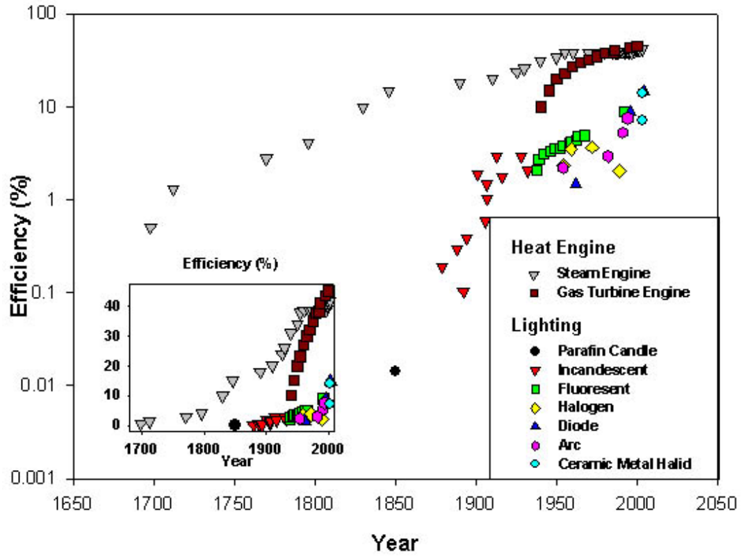
Figure 6 Progress of energy efficiency for heat engines and luminous devices
