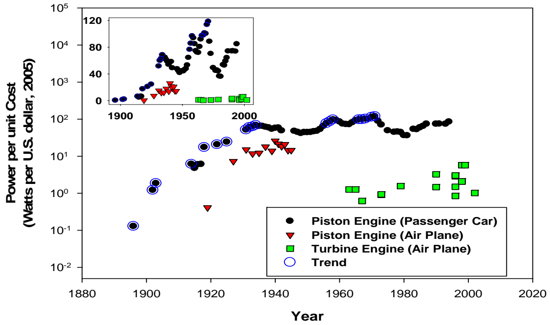
Figure 5 Historical progresses in energy transformation by Power per unit cost (2005) in logarithmic scale
